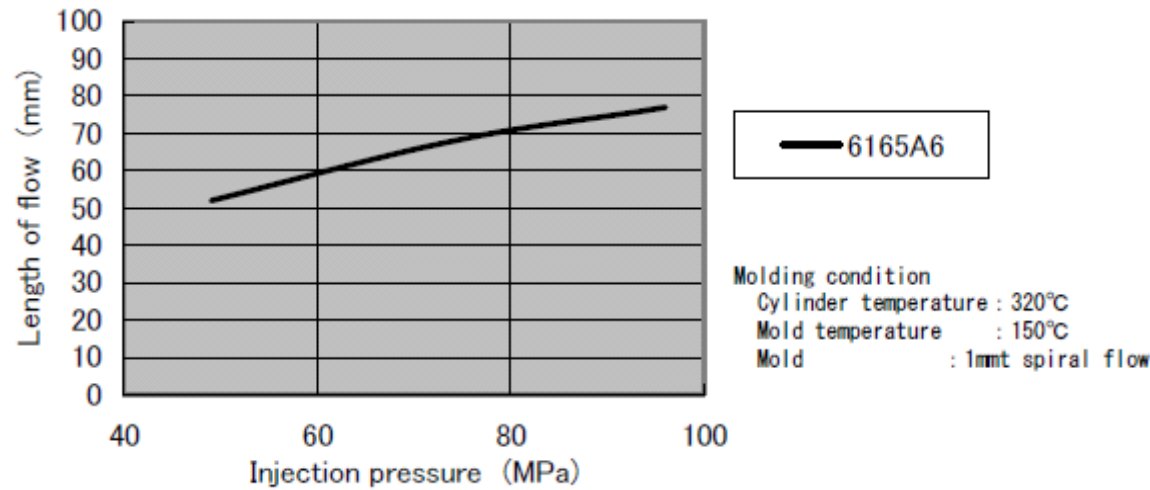
(Figure 3-1) Flowability(1mmt)
