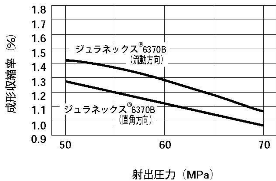
図2-2. 成形収縮率 (120 \square ×2mm t )
