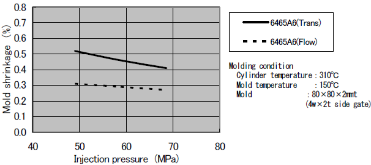
(Figure 4-2) Mold Shrinkage(80□×2mmt)
