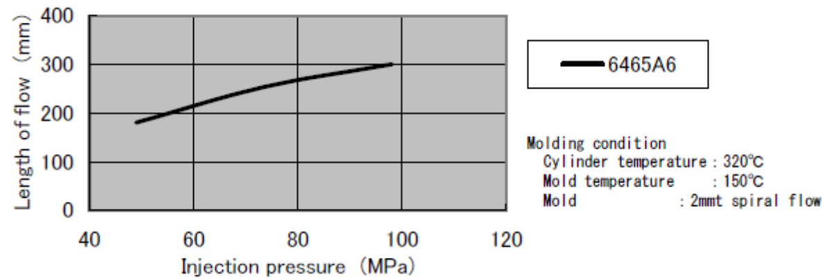
(Figure 3-1) Flowability(2mmt)
