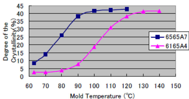
(Figure 3-3) Mold Temperature vs. Degree of the Crystallinity
