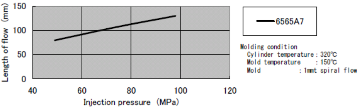
(Figure 3-1) Flowability (1mmt)
