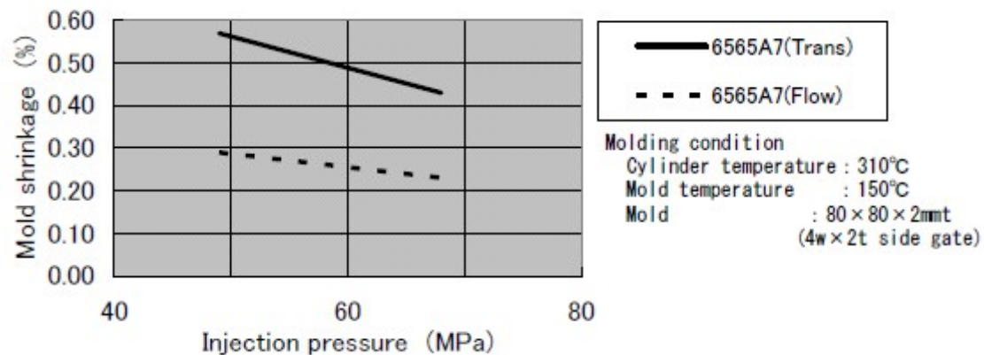
(Figure 3-2) Mold Shrinkage
