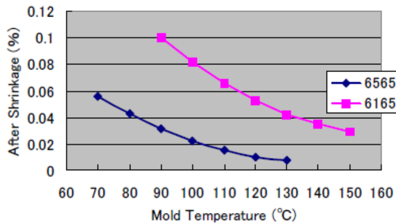
(Figure 3-4) Mold Temperature vs. After Shrinkage
