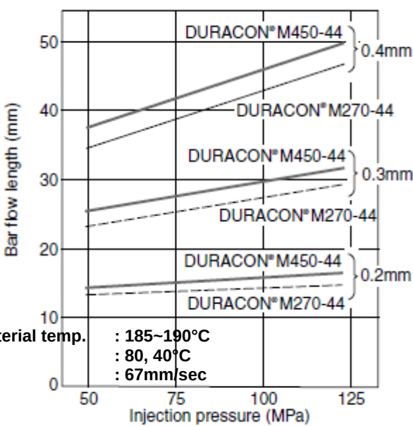
Fig. 2-6 Flowability in case of thin wall (Mold temperature: 40°C)
