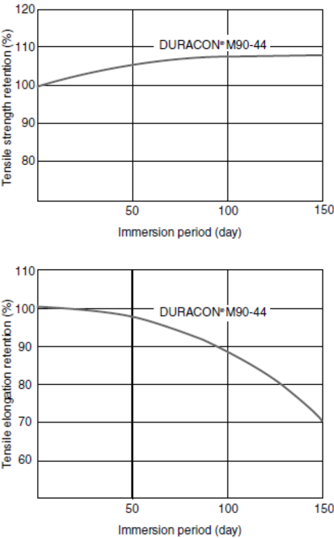
Fig. 1-2 Hot water resistance of DURACON® POM M90-44 (Property retention ratio in 95°C hot water)
