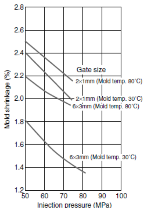
(3) Size of molded parts: 120· 12mm. 3mm thick
