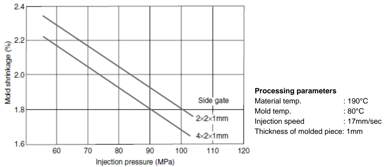
Fig. 2-8 DURACON® POM M270-44 mold shrinkage ratio (Effects of sample thickness and gate size)
