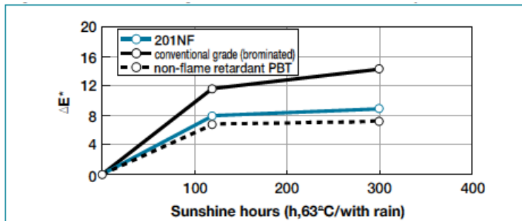
Fig. 3-1 Weather/Light resistance of non-reinforced materials
