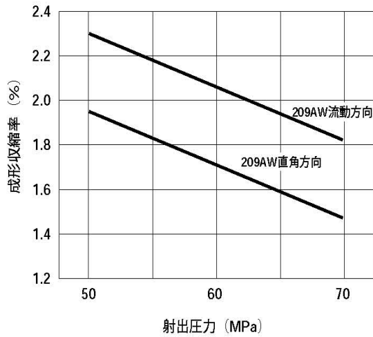
図5 成形収縮率 (120 \square ×2mm \phi )
