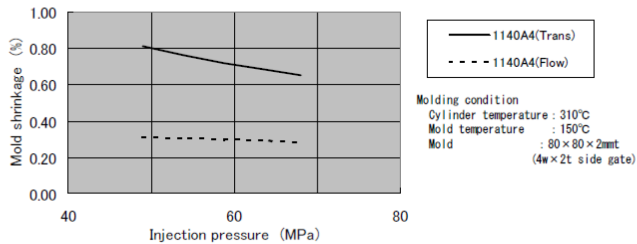
(Figure 3-2) Mold Shrinkage (80□×2mmt)
