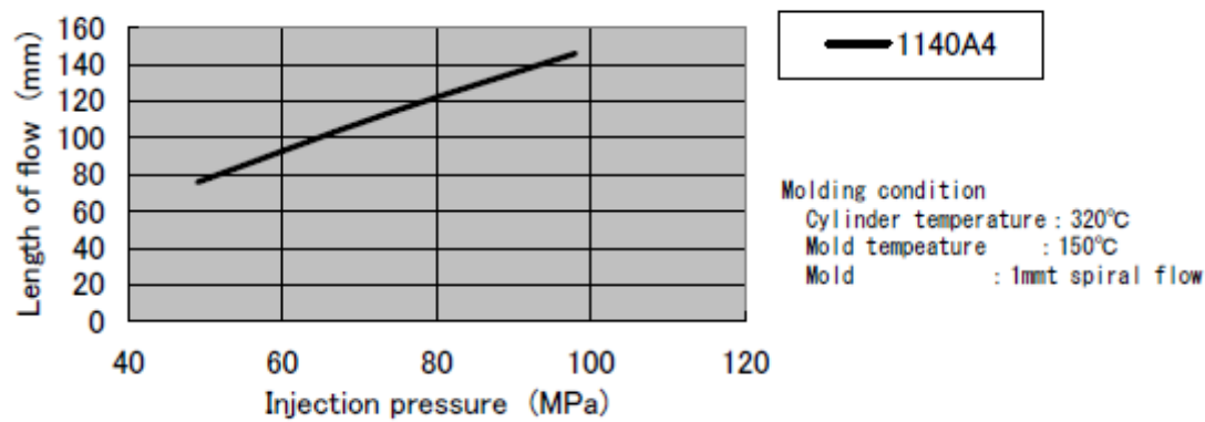
(Figure 3-1) Flowability(1mmt)
